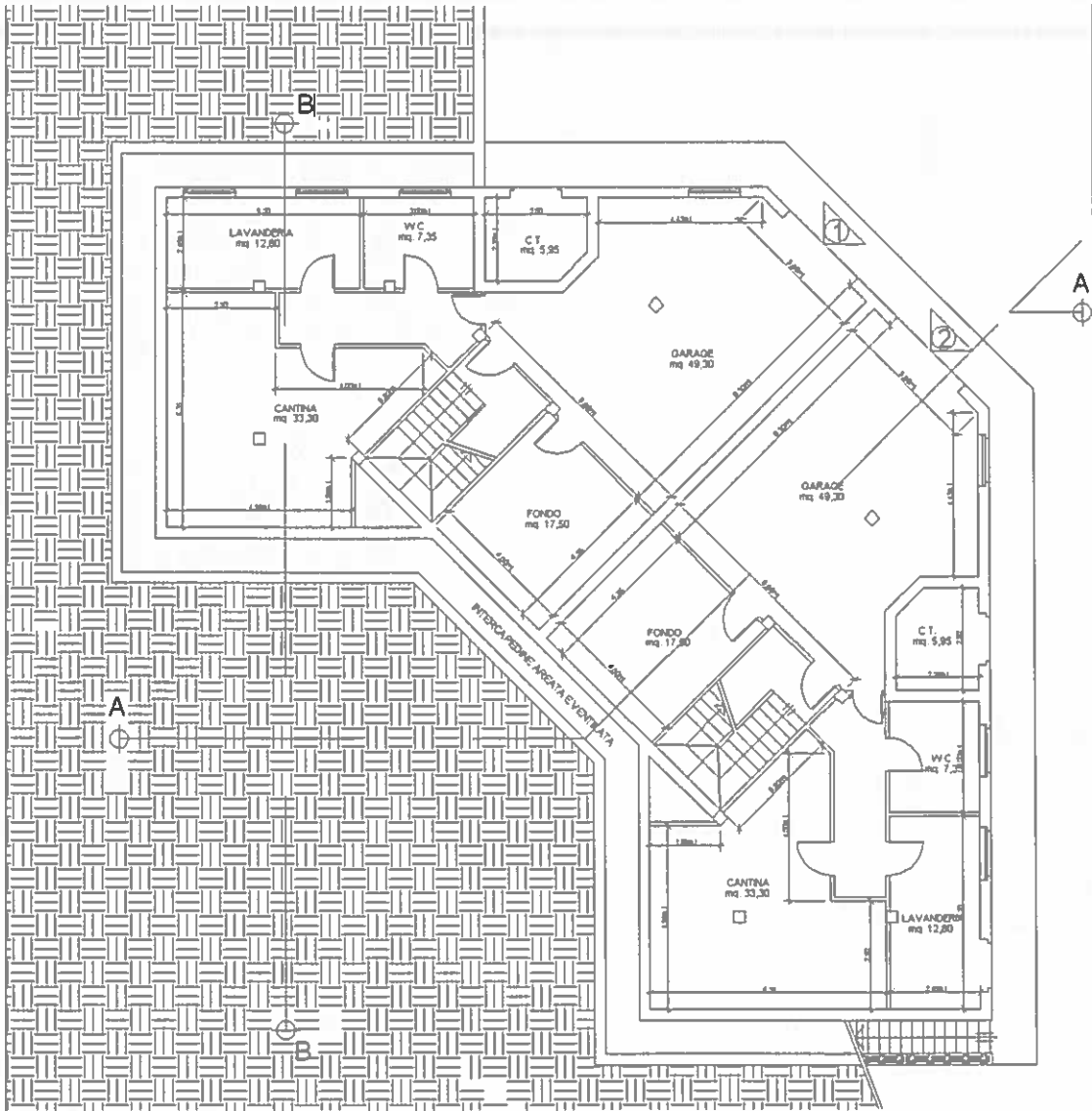
PIANO SEMINTERRATO
