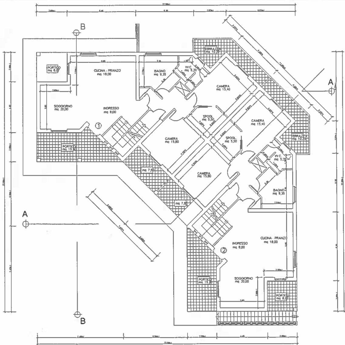
PIANO TERRA
